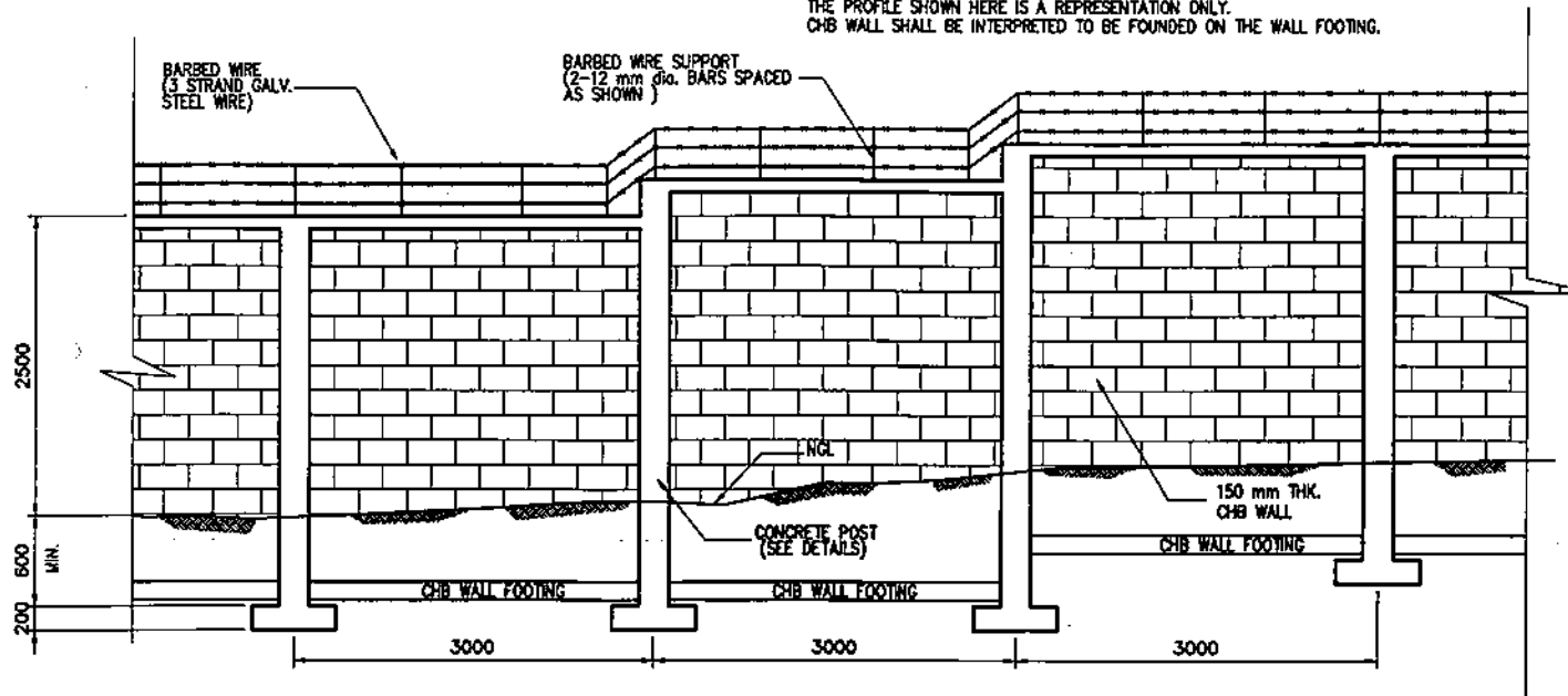
ELEVATION OF CHB FENCE SCALE 1:50
