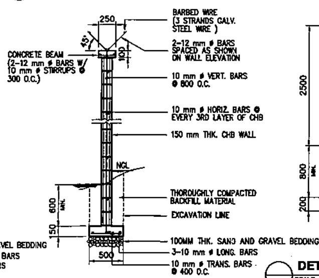
CHB WALL SECTION ON SLOPING GROUND SCALE 1:40
