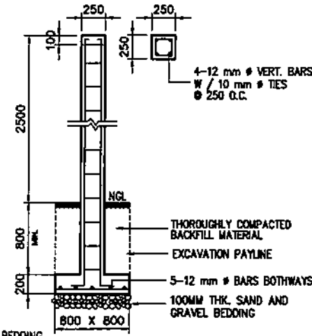
DETAIL OF CONCRETE POST SCALE 1:40
