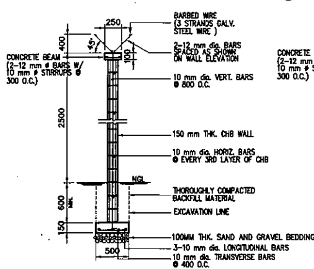
CHB WALL SECTION ON FLAT GROUND SCALE 1:40
